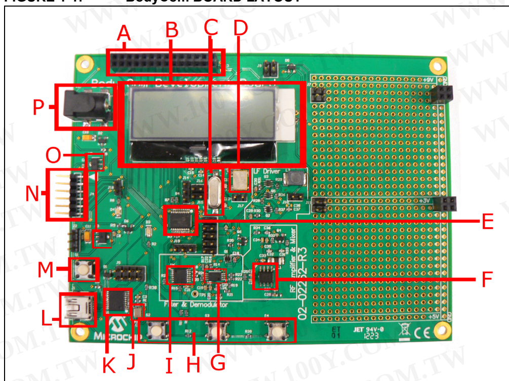
FIGURE 1-1: BodyCom BOARD LAYOUT
