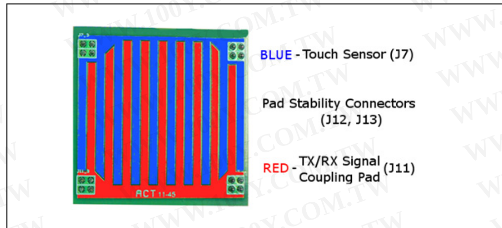
FIGURE 2-3: COUPLING PAD
