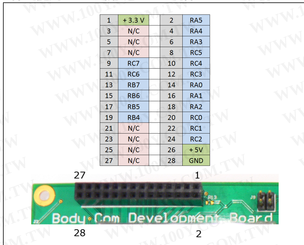
FIGURE 3-1: EXPANSION HEADER CALLOUT
